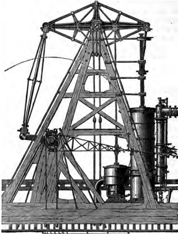
FIG. 180.—Beam-Engine.
